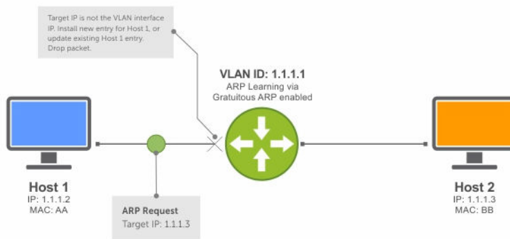
Figure 43. ARP Learning via ARP Request with ARP Learning via Gratuitous ARP Enabled
